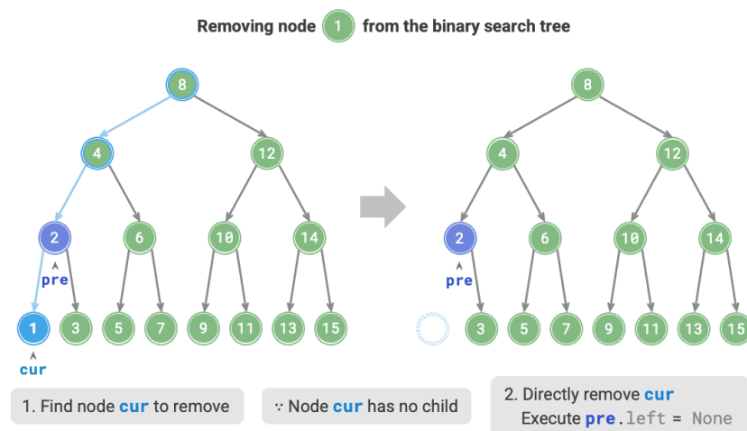
Figure 7-19 Removing a node in a binary search tree (degree 0)
