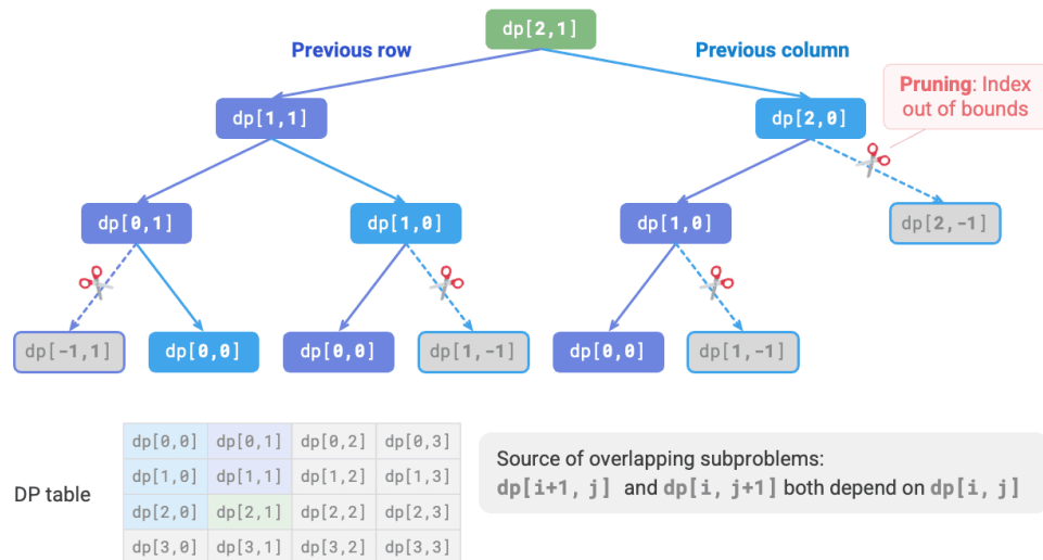
Figure 14-14 Brute force search recursion tree
