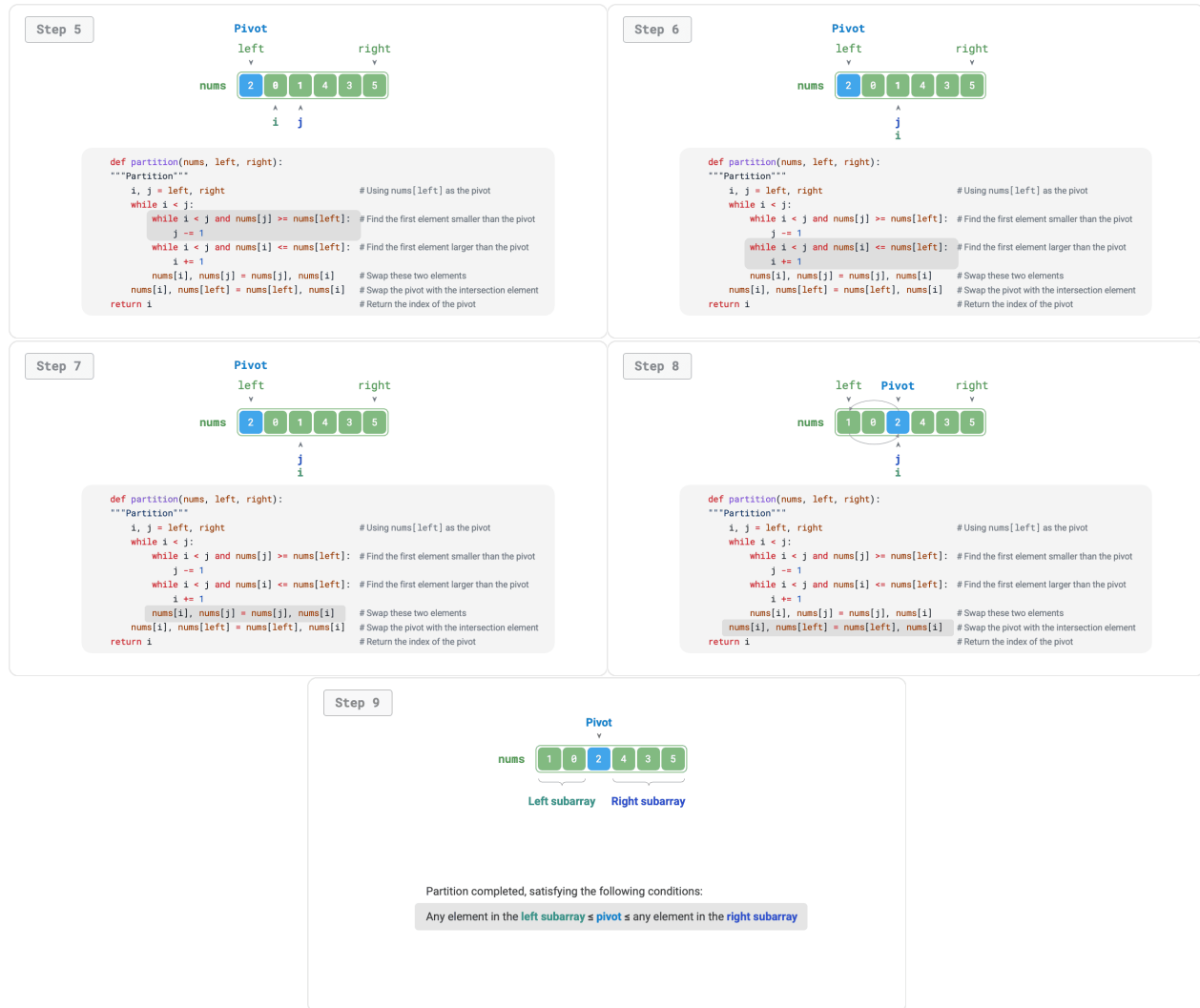
Figure 11-8 Sentinel partitioning steps
