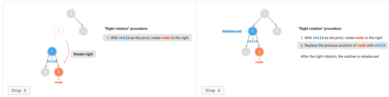
Figure 7-26 Steps of right rotation
