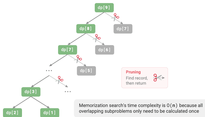
Figure 14-4 Recursion tree with memoization
