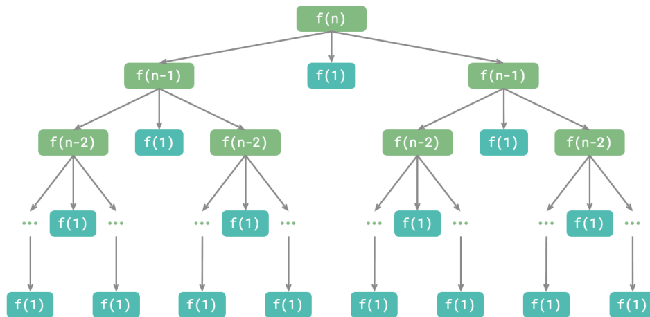
Figure 12-15 Recursion tree of the hanota problem
