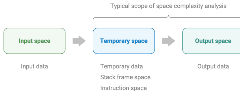
Figure 2-15 Algorithm-related space
