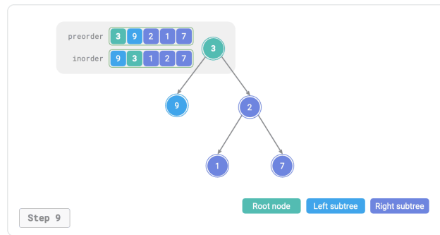
Figure 12-8 Recursive process of building a binary tree
