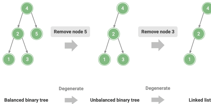
Figure 7-24 Degradation of an AVL tree after removing nodes
