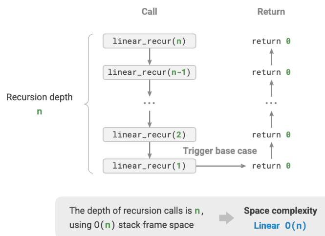
Figure 2-17 Linear order space complexity generated by recursive function
