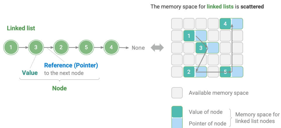
Figure 4-5 Linked list definition and storage method
