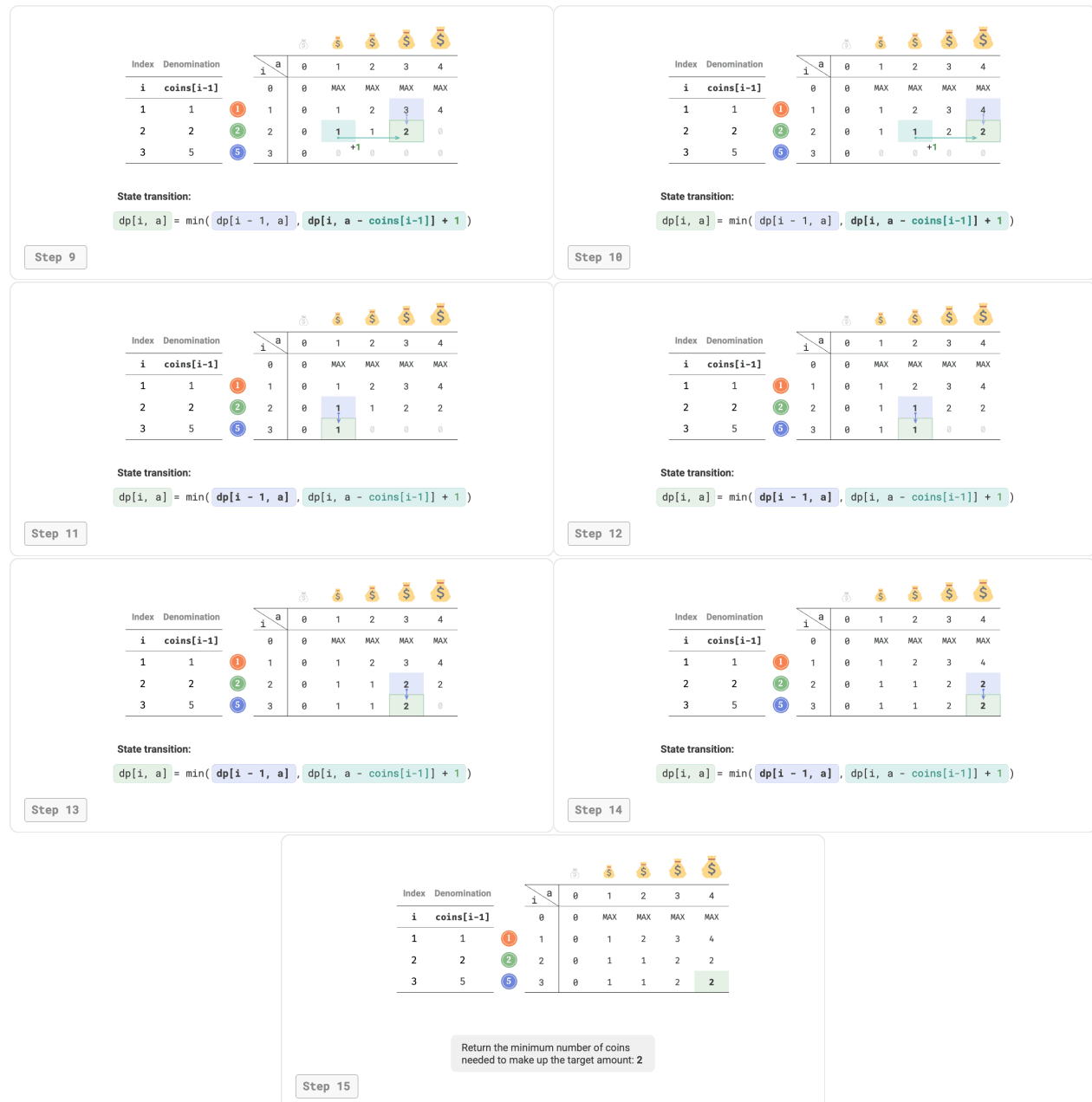
Figure 14-25 Dynamic programming process for coin change problem
