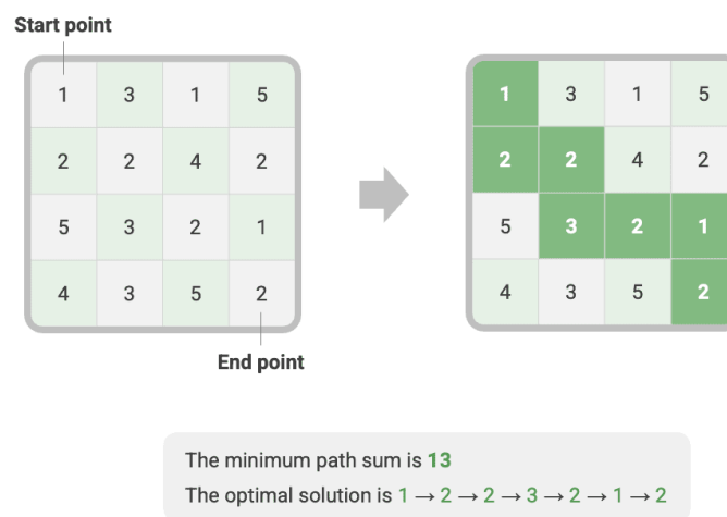
Figure 14-10 Minimum path sum example data
