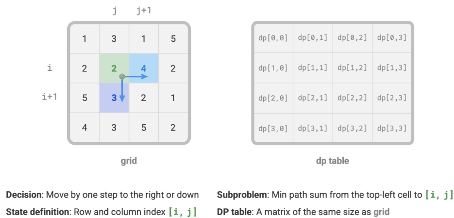
Figure 14-11 State definition and dp table
