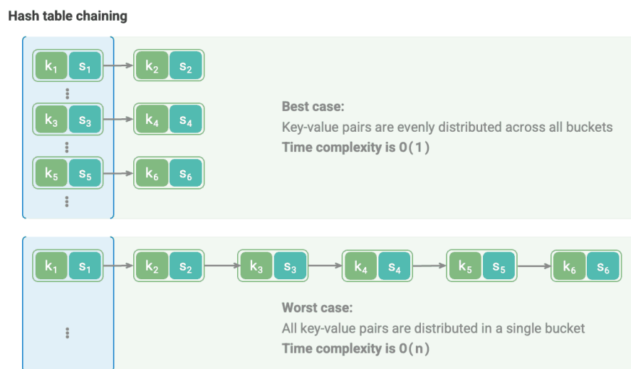
Figure 6-8 Ideal and worst cases of hash collisions
