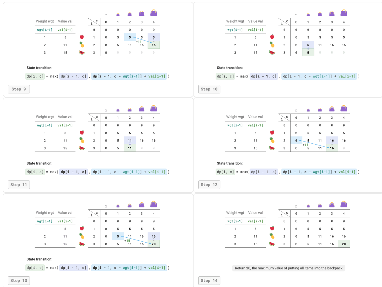
Figure 14-20 Dynamic programming process for 0-1 knapsack problem
