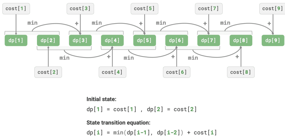
Figure 14-7 Dynamic programming process for climbing stairs with minimum cost
