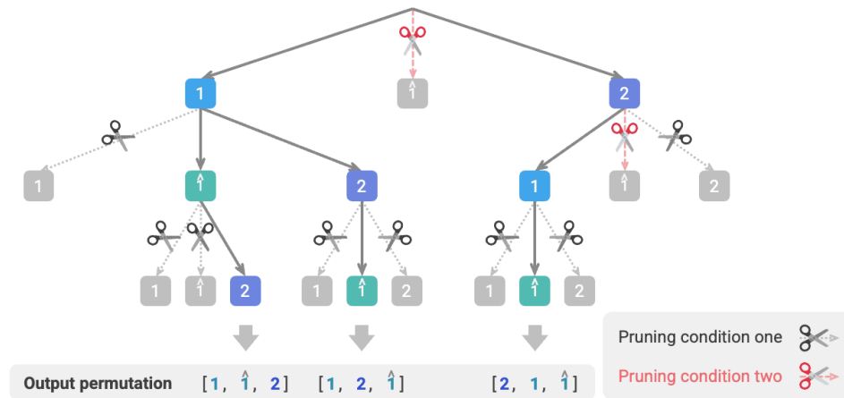
Figure 13-9 Effective scope of two pruning conditions
