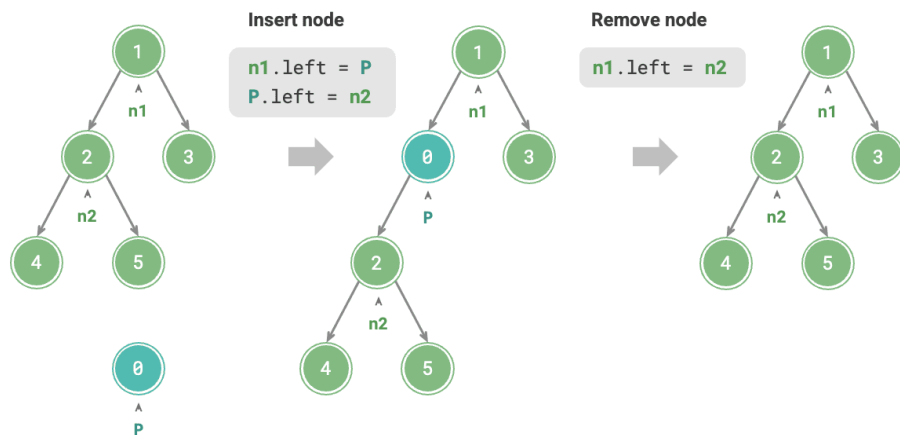
Figure 7-3 Inserting and removing nodes in a binary tree
