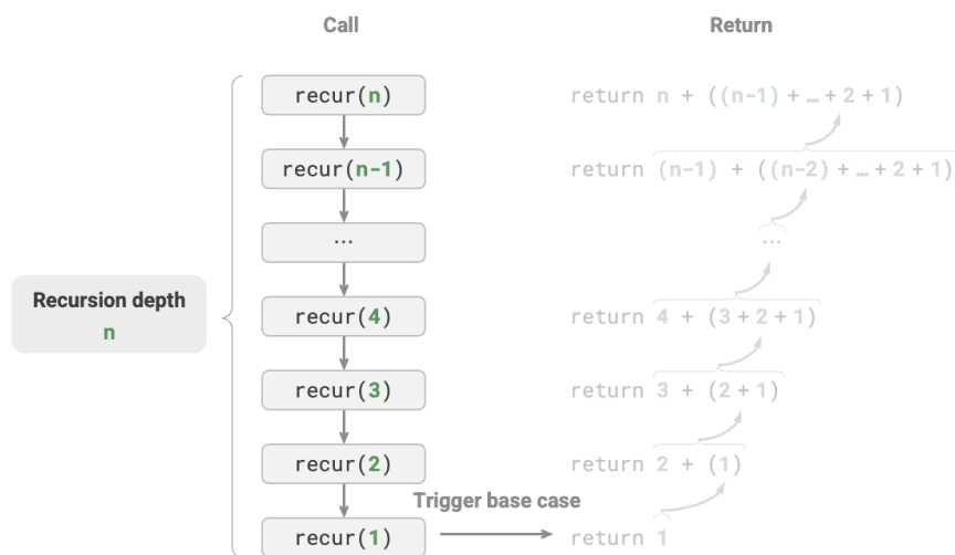
Figure 2-4 Recursion call depth
