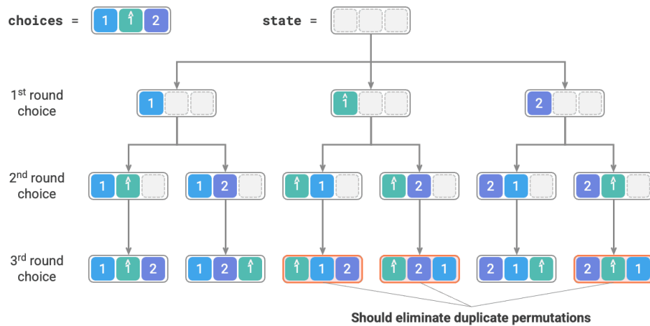
Figure 13-7 Duplicate permutations
