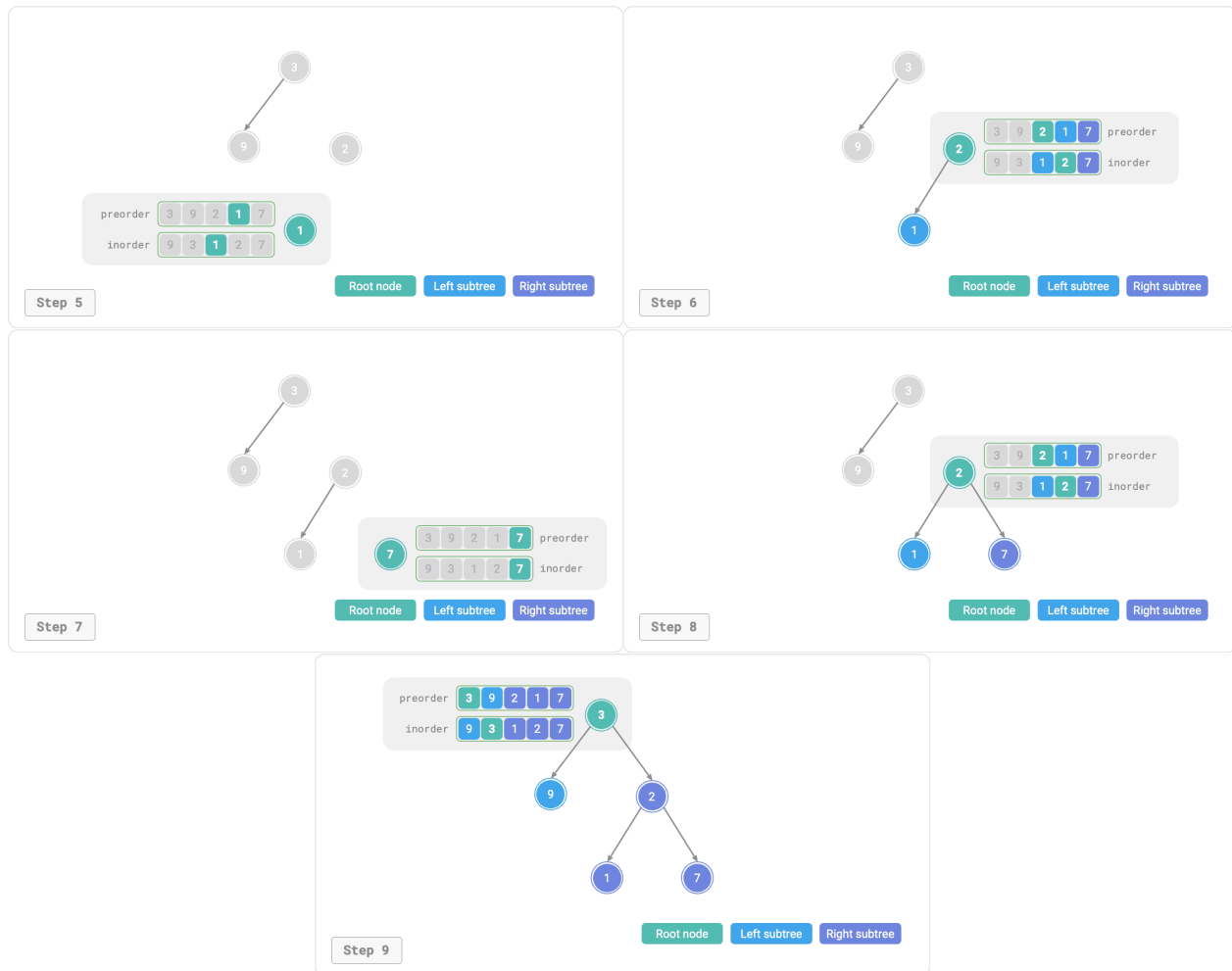
Figure 12-8 Recursive process of building a binary tree
