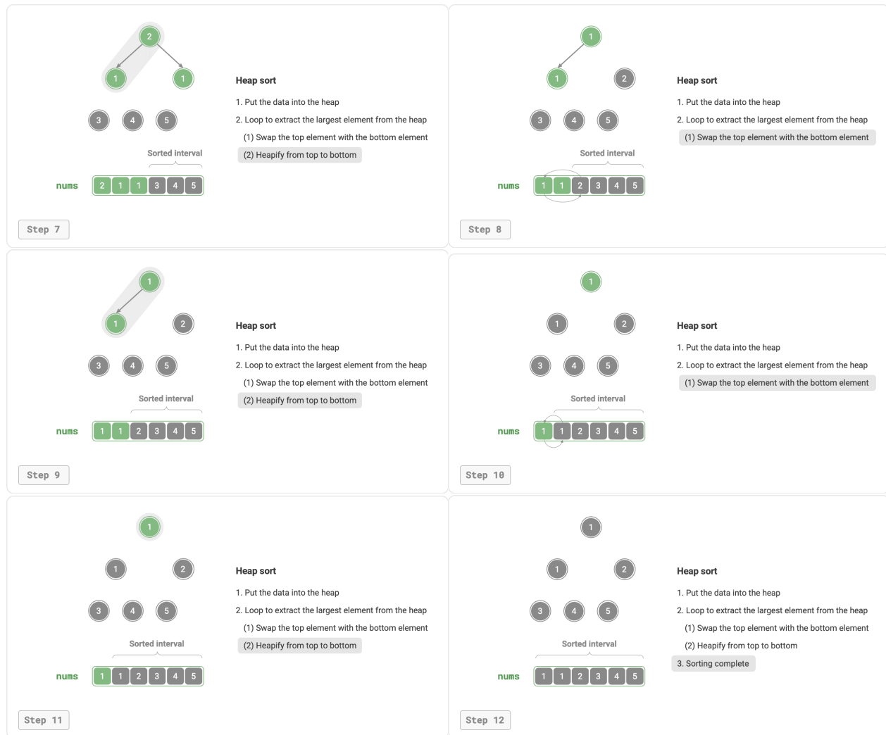
Figure 11-12 Heap sort steps
