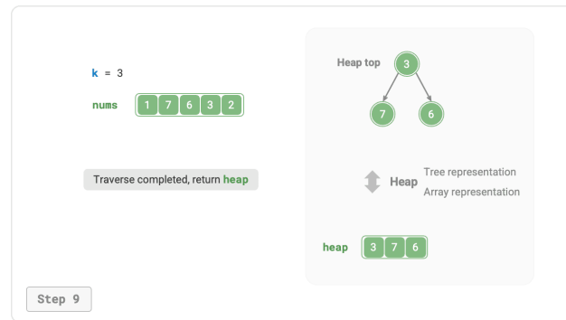
Figure 8-8 Finding the largest k elements using a heap
