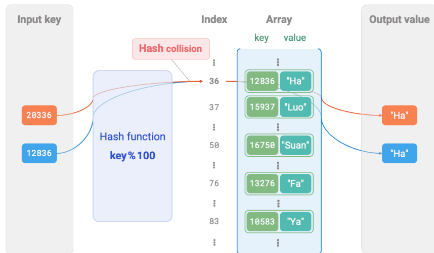
Figure 6-3 Hash collision example
