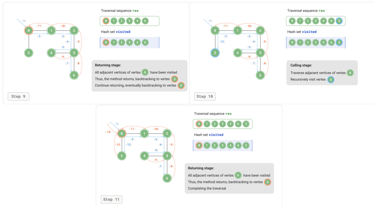
Figure 9-12 Steps of depth-first search of a graph
