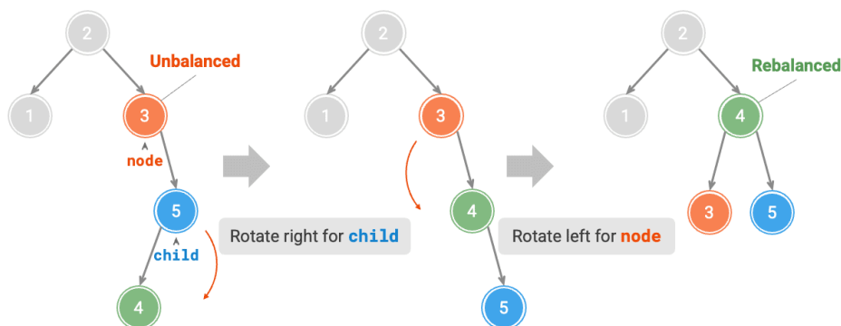
Figure 7-31 Right-left rotation
