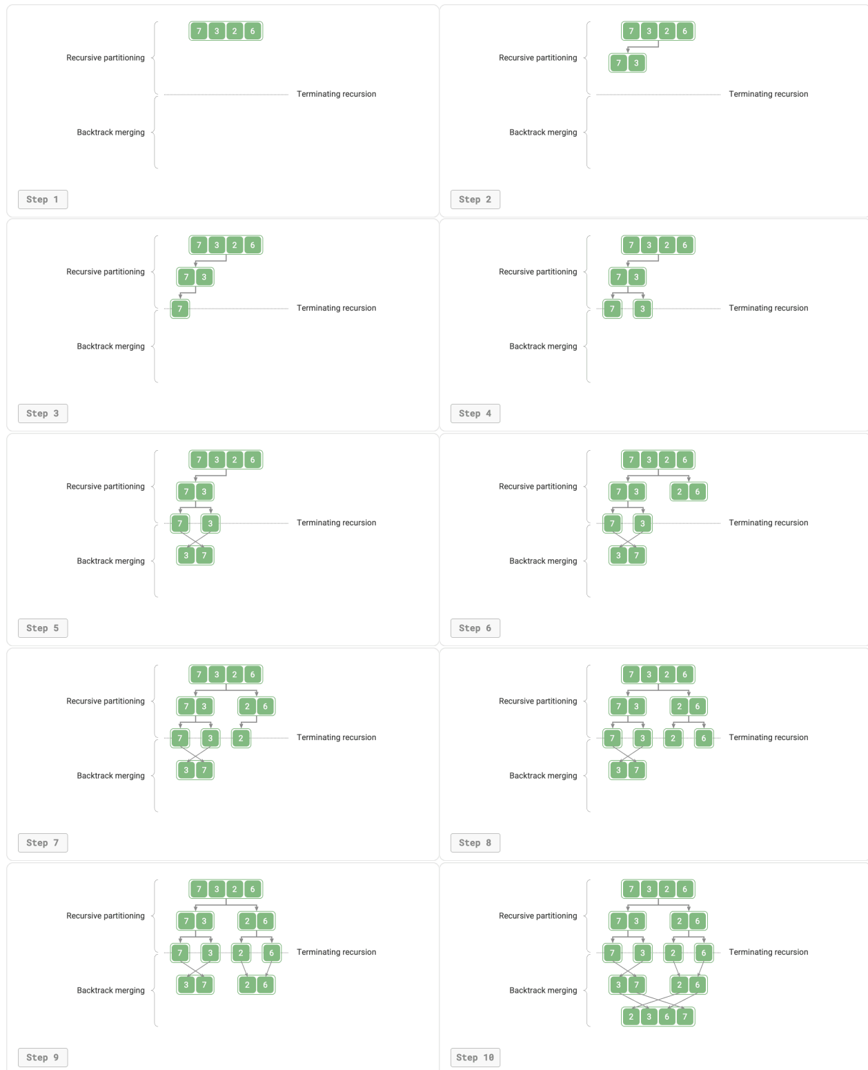
Figure 11-11 Merge sort steps
