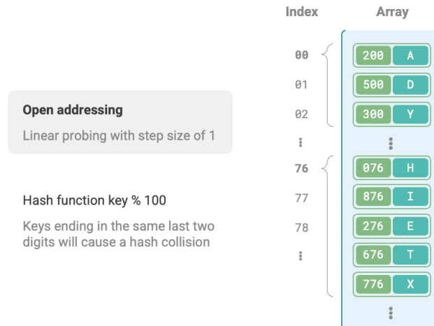
Figure 6-6 Distribution of key-value pairs in open addressing (linear probing) hash table
