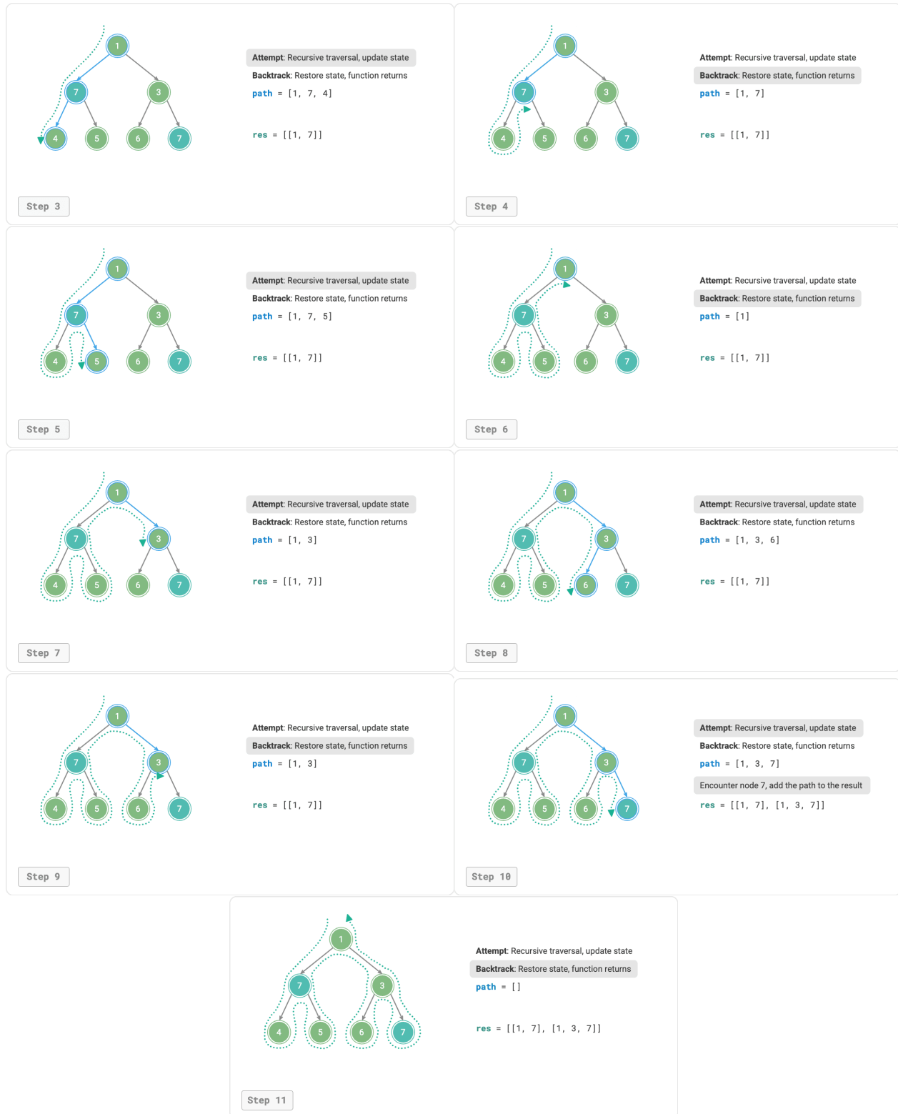
Figure 13-2 Attempt and backtrack
