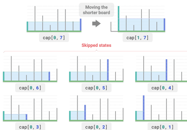
Figure 15-12 States skipped by moving the short partition
