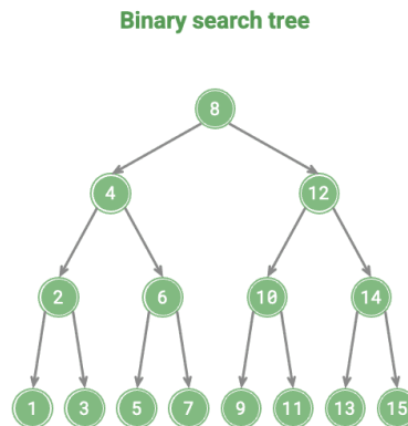
Figure 7-16 Binary search tree
