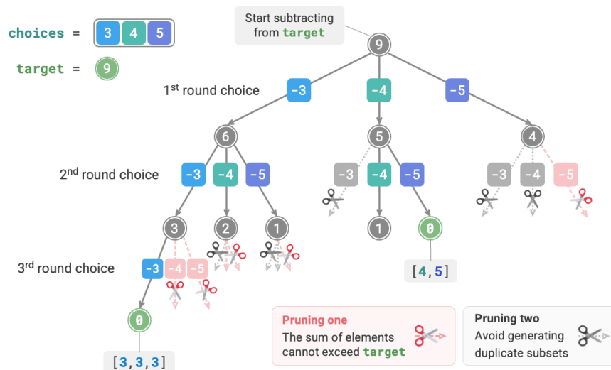
Figure 13-12 Subset-sum I backtracking process
