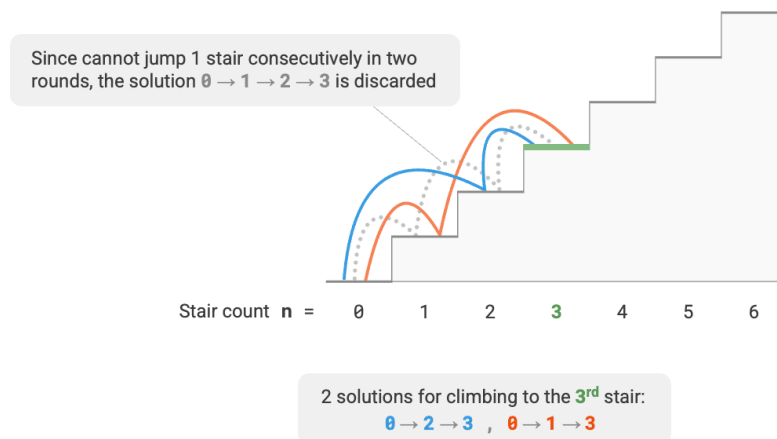
Figure 14-8 Number of ways to climb to the 3rd step with constraint
