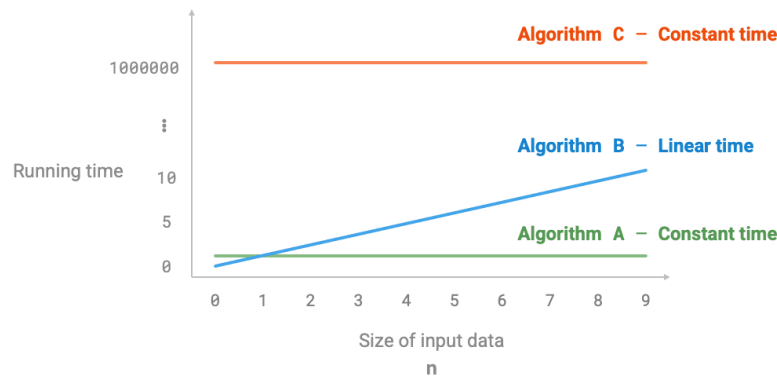
Figure 2-7 Time growth trends of algorithms A, B, and C
