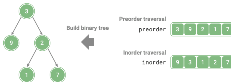
Figure 12-5 Example data for building a binary tree
