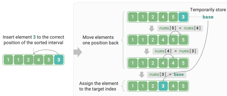
Figure 11-6 Single insertion operation
