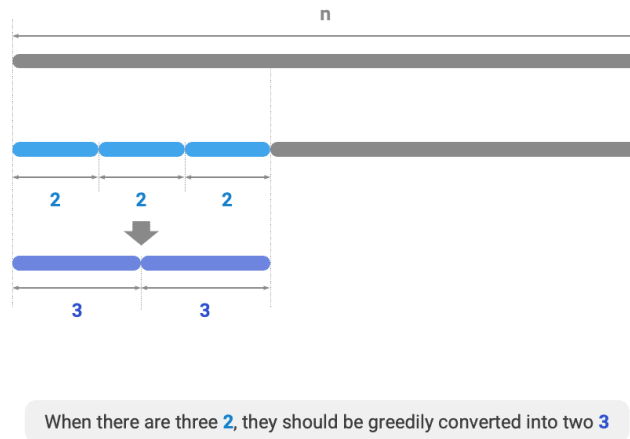
Figure 15-15 Optimal splitting factor
