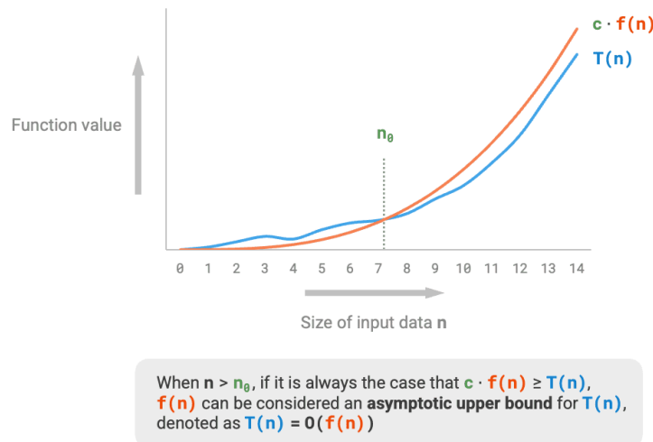
Figure 2-8 Asymptotic upper bound of a function
