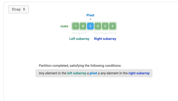
Figure 11-8 Sentinel partitioning steps
