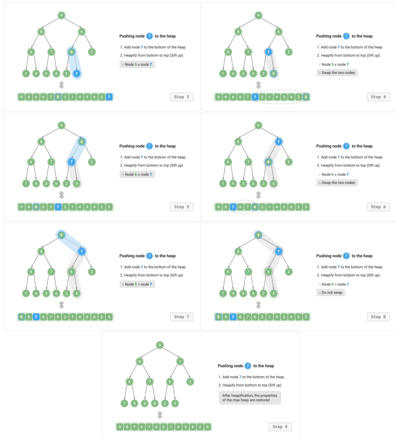
Figure 8-3 Steps of inserting an element into the heap
