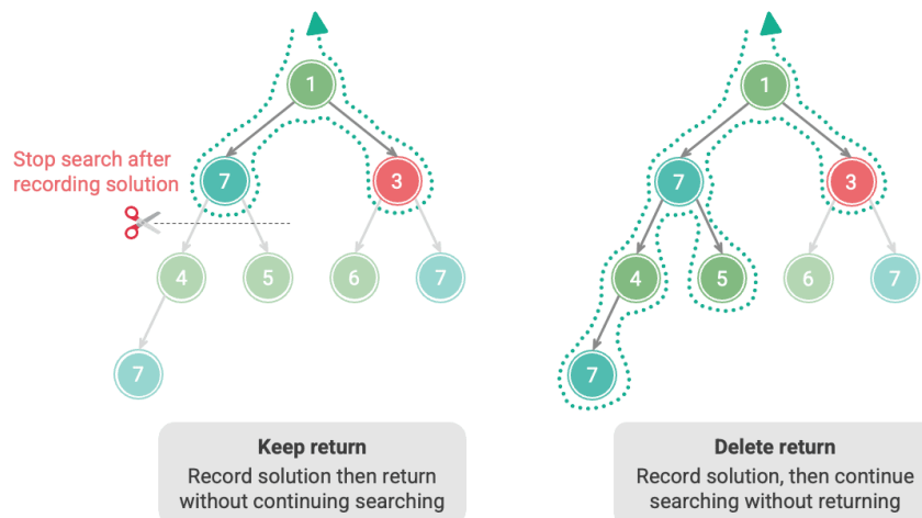
Figure 13-4 Comparison of search process with and without return statement
