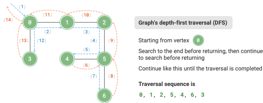
Figure 9-11 Depth-first search of a graph
