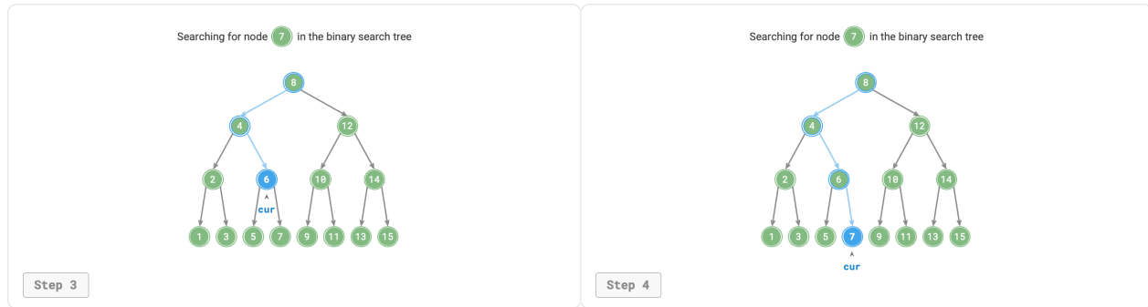
Figure 7-17 Example of searching for a node in a binary search tree
