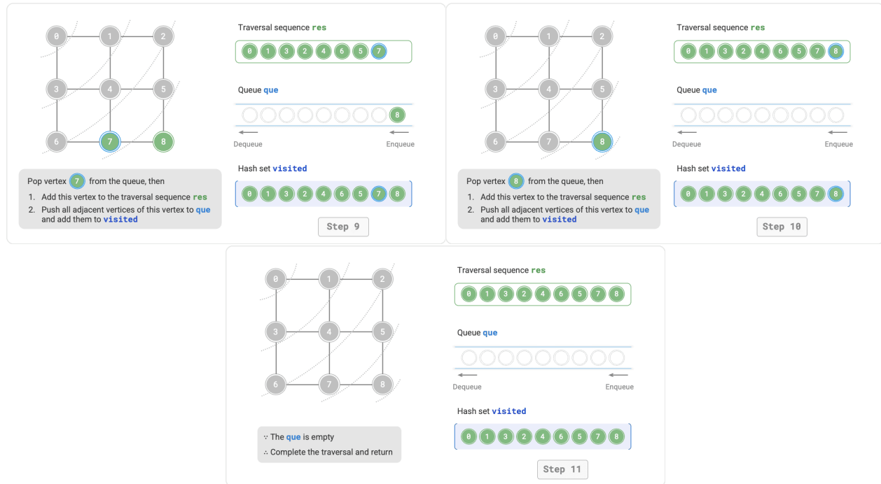
Figure 9-10 Steps of breadth-first search of a graph
