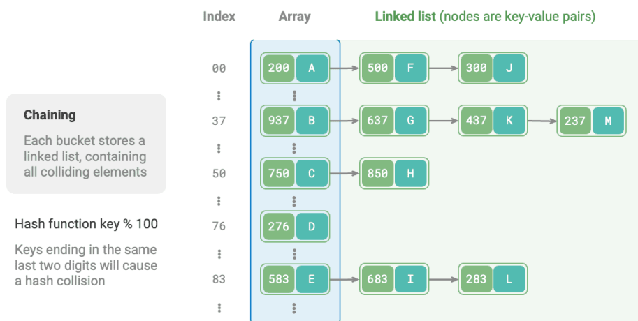
Figure 6-5 Separate chaining hash table
