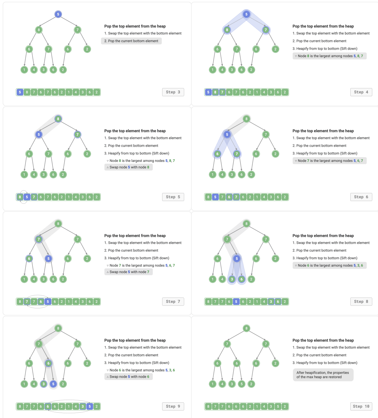
Figure 8-4 Steps of removing the heap top element
