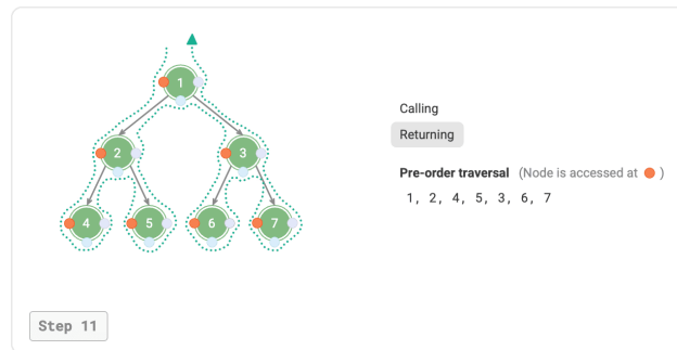
Figure 7-11 The recursive process of preorder traversal
