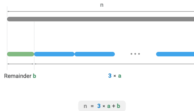
Figure 15-16 Calculation method for max product cutting
