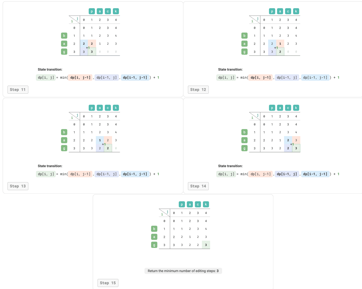
Figure 14-30 Dynamic programming process for edit distance
