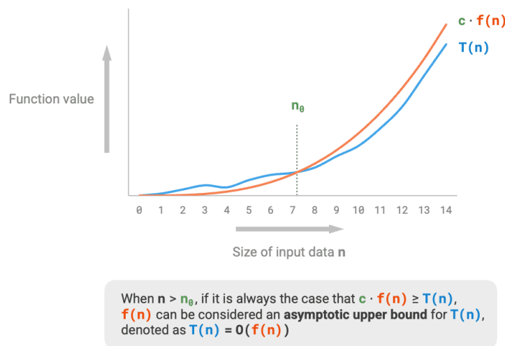
Figure 2-8 Asymptotic upper bound of a function
