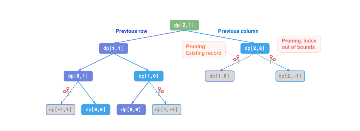
Figure 14-15 Memoization recursion tree
