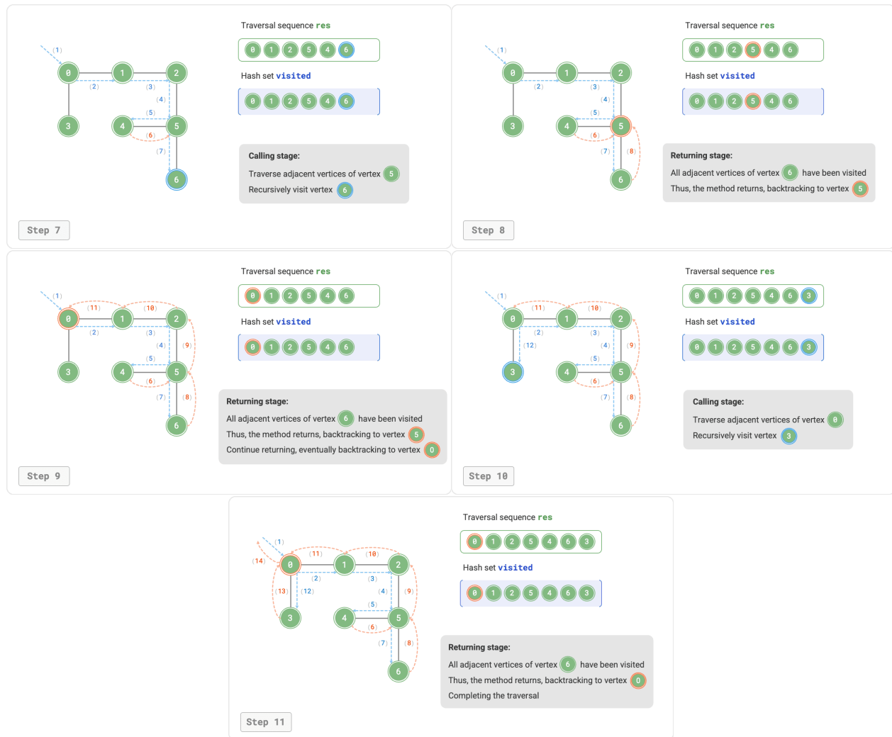
Figure 9-12 Steps of depth-first search of a graph
