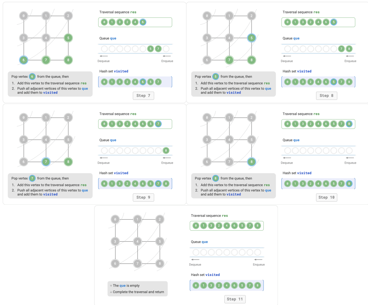
Figure 9-10 Steps of breadth-first search of a graph
