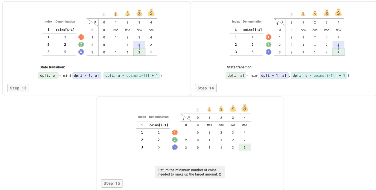
Figure 14-25 Dynamic programming process for coin change problem
