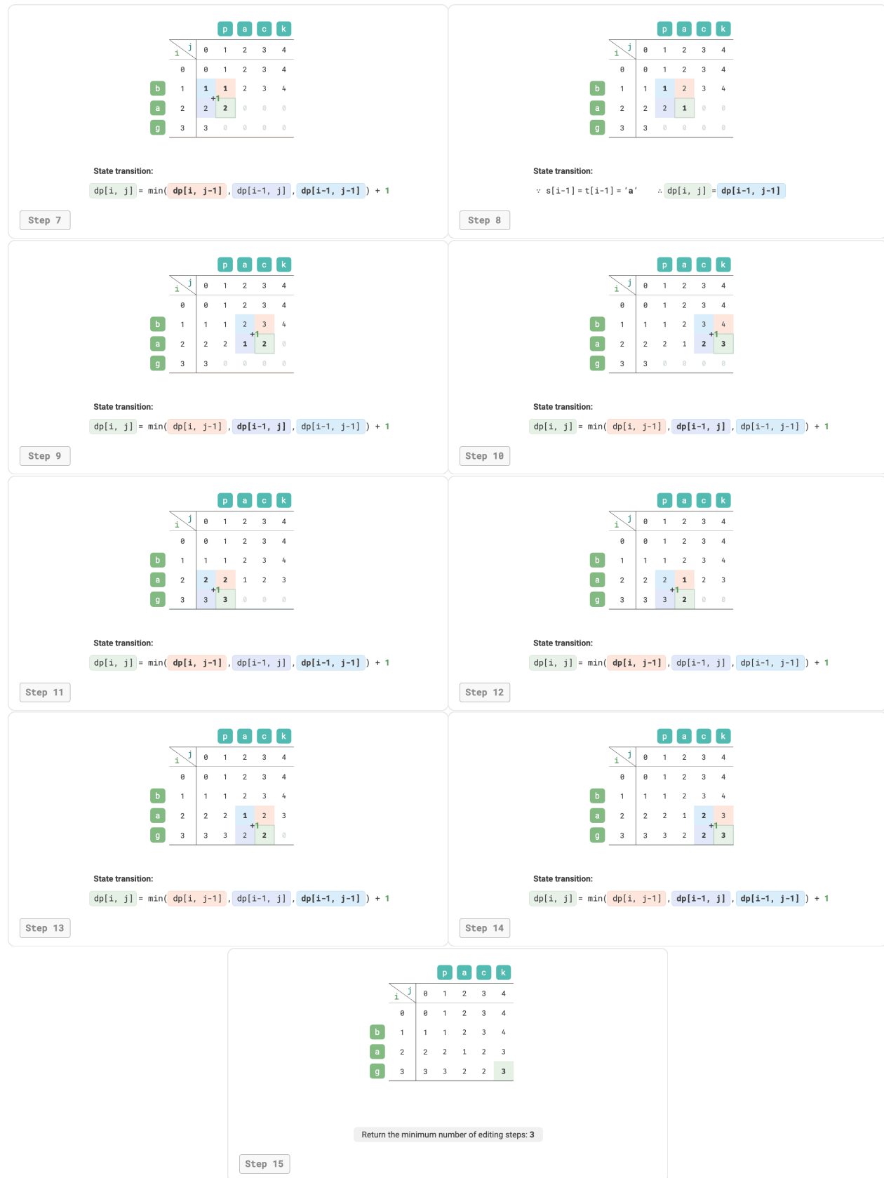
Figure 14-30 Dynamic programming process for edit distance
