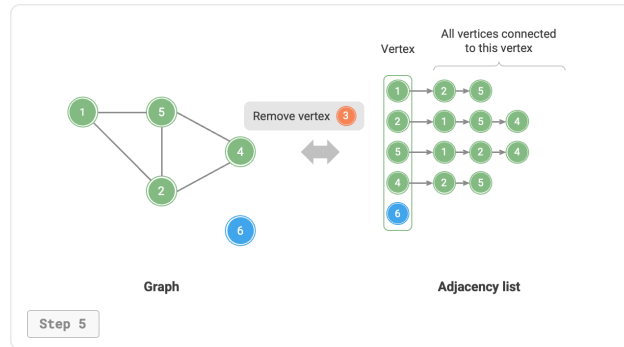
Figure 9-8 Initialization, adding and removing edges, adding and removing vertices in adjacency list
