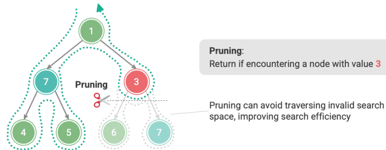
Figure 13-3 Pruning according to constraints
