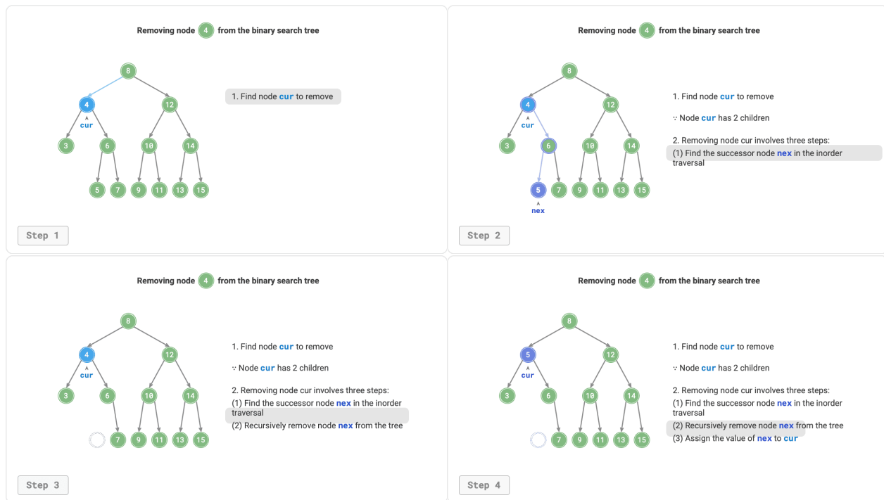
Figure 7-21 Removing a node in a binary search tree (degree 2)
