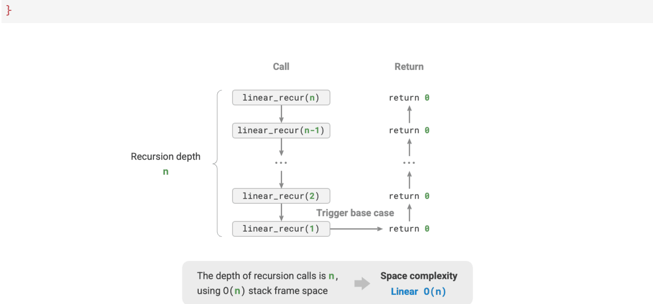
Figure 2-17 Linear order space complexity generated by recursive function
