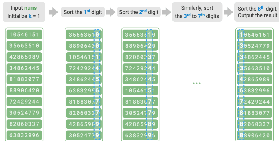
Figure 11-18 Radix sort algorithm flow
