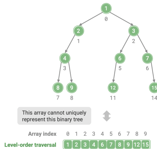
Figure 7-13 Level-order traversal sequence corresponds to multiple binary tree possibilities
