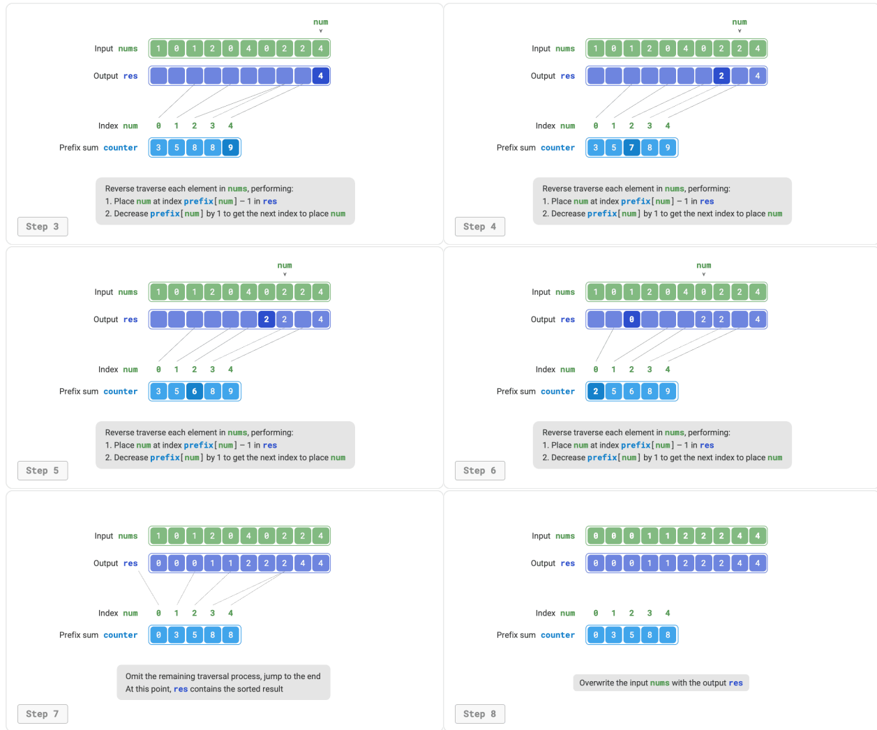
Figure 11-17 Counting sort steps
