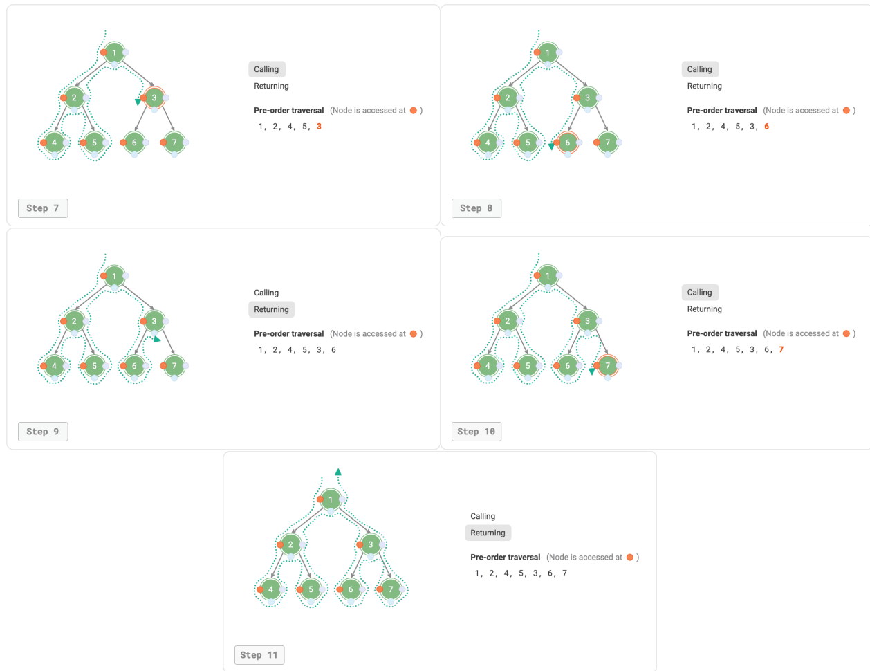
Figure 7-11 The recursive process of preorder traversal
