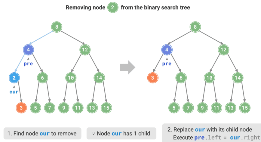
Figure 7-20 Removing a node in a binary search tree (degree 1)
