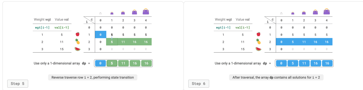
Figure 14-21 Space-optimized dynamic programming process for 0-1 knapsack
