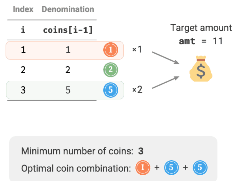
Figure 14-24 Example data for coin change problem
