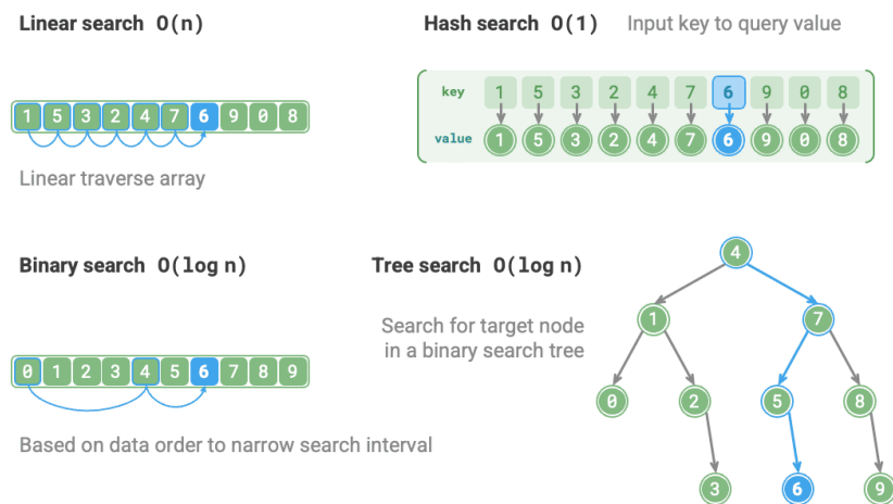
Figure 10-11 Multiple search strategies
