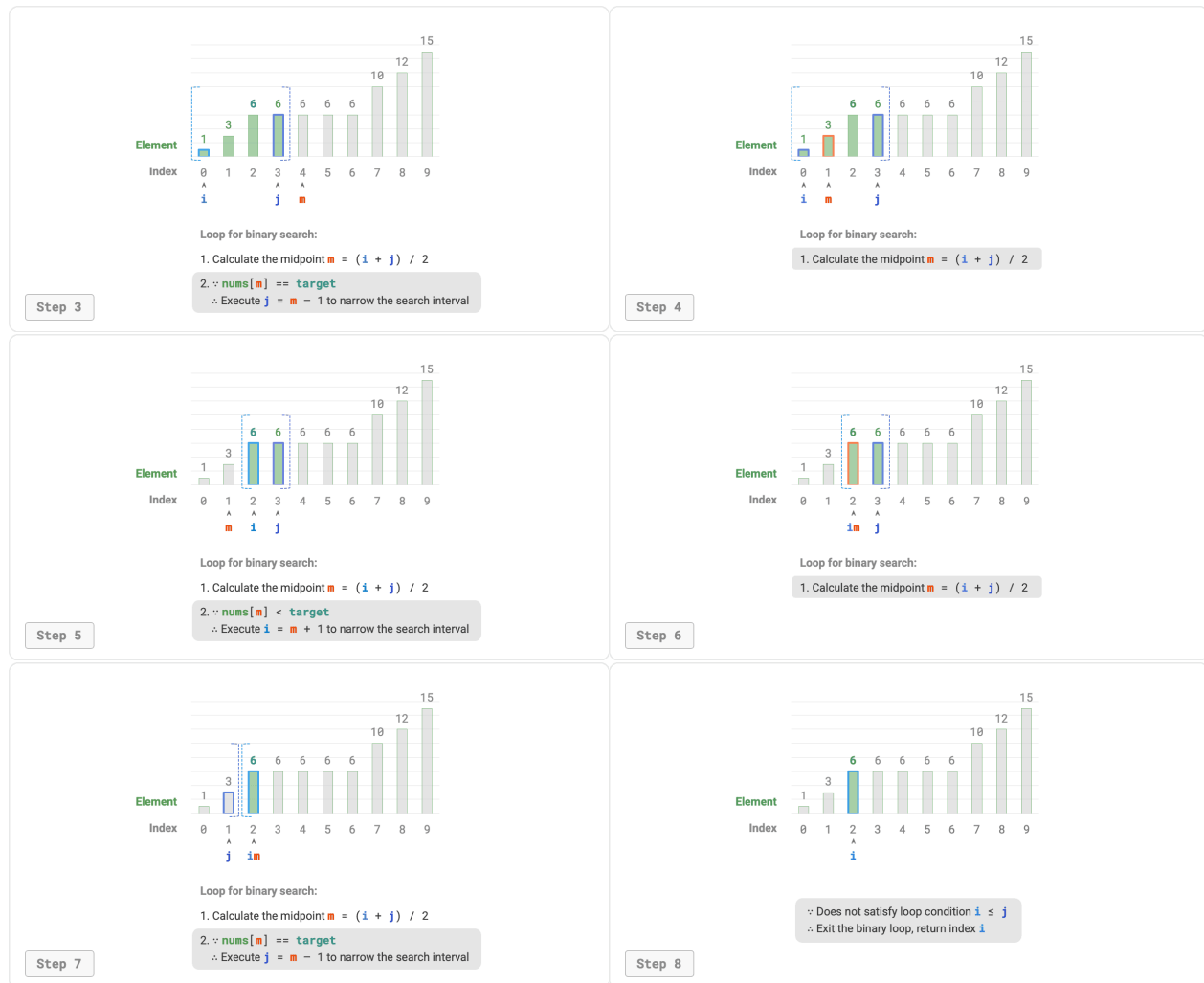
Figure 10-6 Steps for binary search insertion point of duplicate elements
