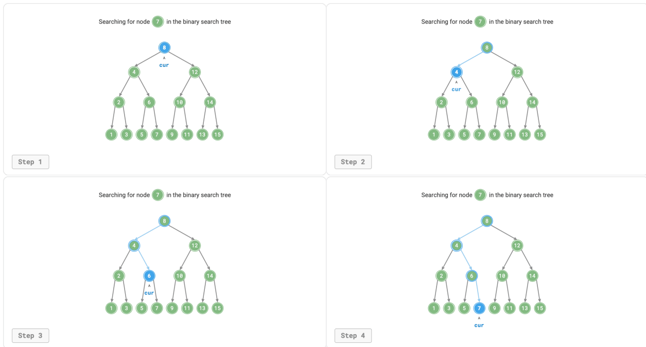
Figure 7-17 Example of searching for a node in a binary search tree
