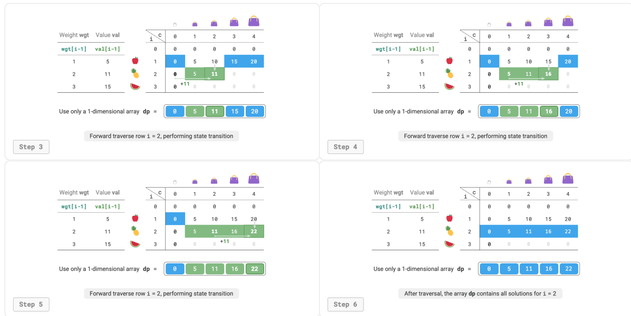
Figure 14-23 Space-optimized dynamic programming process for unbounded knapsack problem
