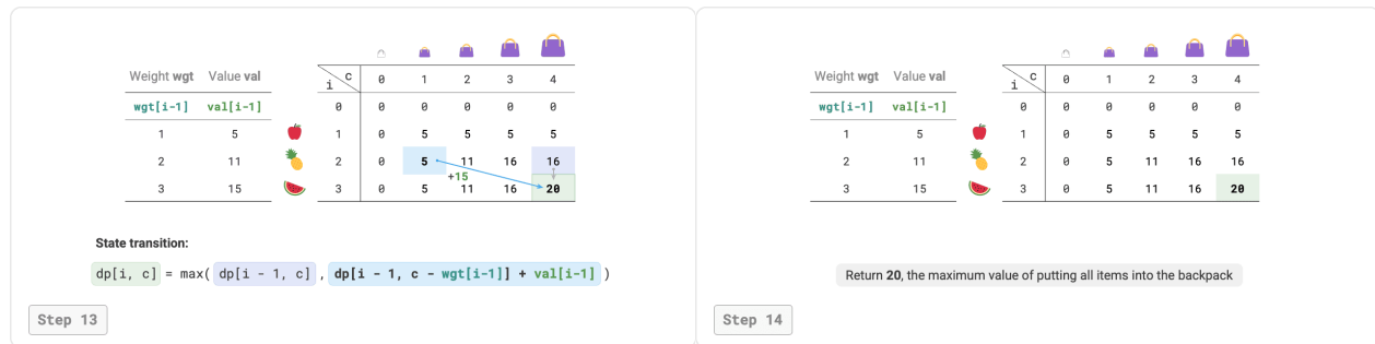
Figure 14-20 Dynamic programming process for 0-1 knapsack problem
