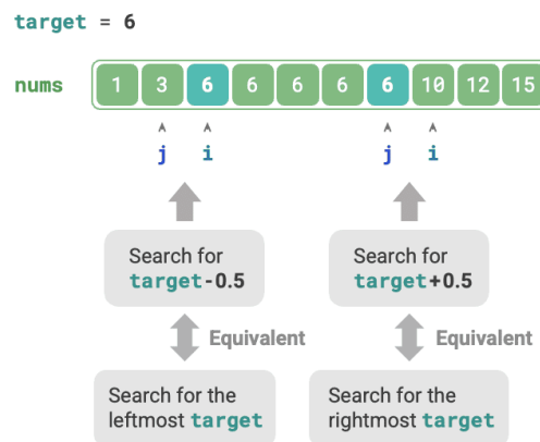
Figure 10-8 Converting boundary search to element search
